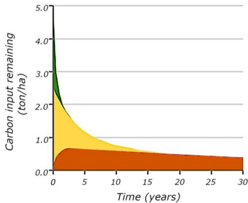
Figure 1: Illustration of the fate of plant organic inputs into a soil (single input event, here 5 t Cha -1 ). The numerical values are representative of the 0–30 cm layer of temperate soils. In this diagram, the mineralization kinetics is arbitrarily divided into three phases: fast, intermediate and slow. Organic matter can be divided into three corresponding pools, the size of which is represented in the figure by the coloured areas. (Modified from Pellerin et al., 2020; Basile-Doelsch et al., 2020).
