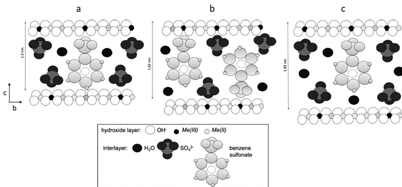
Fig. 7. Possible interlayer arrangement of benzene sulfonate (BzS) in the green rust structure. Calculated basal spacing is shown for each structure: (a) monolayer with dehydrated BzS in a single direction; (b) monolayer with dehydrated BzS moieties facing away from each other and (c) monolayer with hydrated BzS in a single direction, modified from Perez et al. (2018).
