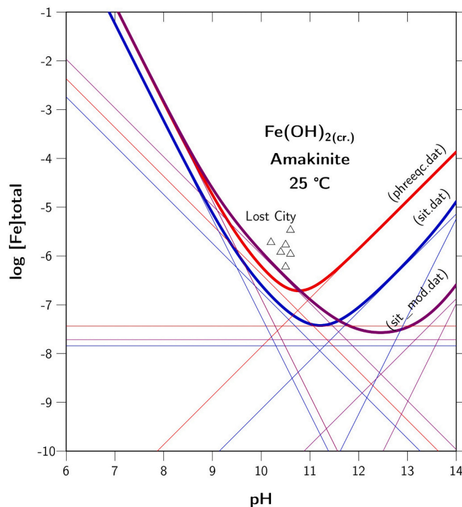
Fig. 10. Lost City hydrothermal fluid compositions (open triangles) as reported in the solubility diagram of ferrous hydroxide \text{Fe}(\text{OH})_2(\text{cr}) amakinite at 25^\circ\text{C} , and for pH values given at 25^\circ\text{C} in Seyfried et al. (2015). Curves, also computed at 25^\circ\text{C} correspond to the three different values of solubility of amakinite at elevated pH found in the currently available databases, namely phreeqc.dat, sit.dat and modified sit.dat and new experimental data (Ben Nacib et al., 2016; Ben Nacib, 2017). The uncertainties on iron speciation at \text{pH} > 11 , expressed in the three solubility curves, have no bearing; pH should be lower than 9 where temperature is higher, e.g., in the root of the hydrothermal system (Seyfried et al., 2015), hence in the diagram region where all solubility curves are very close to each other.
