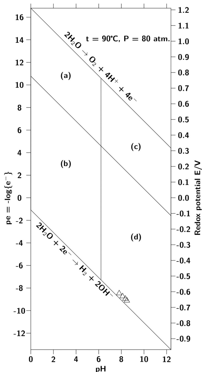
Fig. 9. Lost City hydrothermal fluids composition (open triangles) in the stability domain of water expressed as (pe, pH) at temperature t = 90^\circ\text{C} , and pressure P = 80\text{ atm} . The corresponding ion-product constant of liquid water ( K_w ), defined as K_w = \{H^+\}\{OH^-\} , is such that \log K_w = -12.38 ; (a) oxidizing – acid; (b) reducing – acid; (c) oxidizing – alkaline; (d) reducing – alkaline conditions; upper oxidizing limit, pe + pH = 16.80 ; lower reducing limit, pe + pH = -1.08 .
