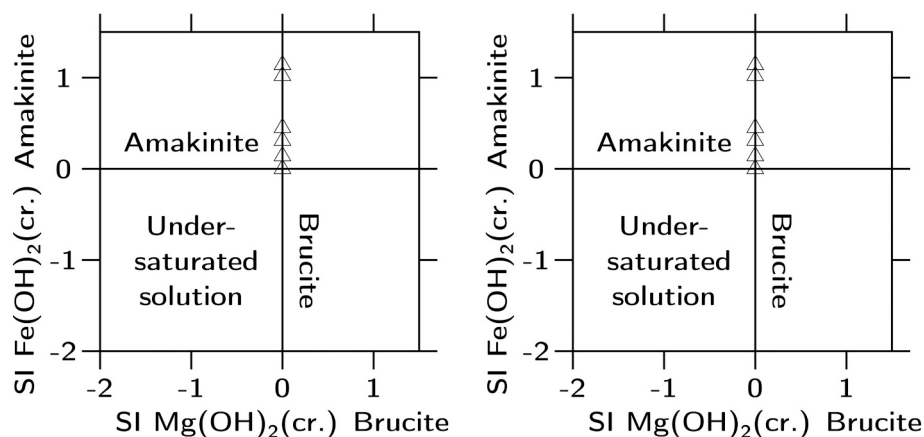
Fig. 11. Lost City hydrothermal fluid compositions (open triangles) in the equilibrium diagram Fe(OH) 2 (cr.) amakinite - Mg(OH) 2 (cr) brucite. The same data are plotted under two different assumptions: left: when solutions are forced to equilibrium with brucite; right: when solutions are forced to equilibrium with amakinite. SI stands for saturation index (Table 3).
