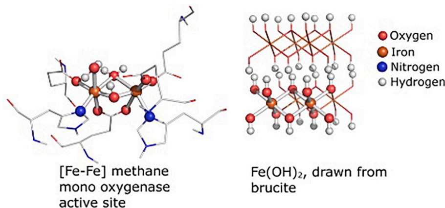
Fig. 1. Structural analogy between the active site of the soluble form of methane monooxygenase and the ferrous hydroxide amakinite (or “ferroan brucite”), a structural component of the brucitic layer of fougerite, a mixed ferrous and ferric hydroxide. A \mu_2 -OH bond, with 2 OH ligands doubly bridging iron atoms is common to the active site of the enzyme and to amakinite octahedral layer, reproduced from Nitschke et al. (2013) (For interpretation of the colours in this figure, the reader is referred to the web version of this article.)
