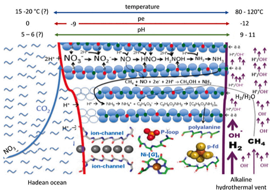
Fig. 2. Interaction fougérite-milieu and resulting reactions in the interlayers in alkaline hydrothermal vents, modified from Russell (2018).
