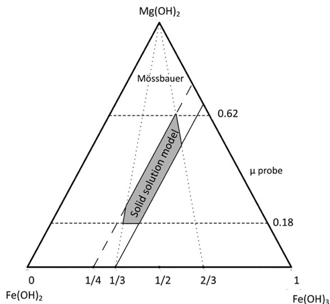
Fig. 5. Composition stability domain of fougèrite from Fougères (in grey) from Trolard et al. (2007). It is derived from a solid solution model (shown with solid and long dashed lines) constrained by Fe(III)/Fe total ratio comprised between 1/4 and 1/3, the Mg/Fe total mole ratio comprised between 0.18 and 0.62, and the Fe(III)/(Fe total + Mg) mole ratio determined by electron microprobe analysis ( \mu -probe: short dashed lines) and Mössbauer spectroscopy (dotted lines).
