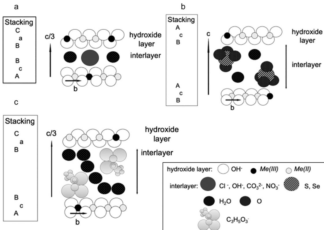
Fig. 4. Stacking sequences and structures of layered double hydroxides (modified from Trolard and Bourrié (2012) and Sabot et al. (2007)). For green rusts, M(II) = Fe(II) and M(III) = Fe(III); Panel (a) corresponds to GR1 structure, panel (b) to GR2 structure and panel (c) to GR-lactate structure; Note that only the main interlayer anions are shown in the drawings of the structure; a , b and c correspond to unit cell dimensions; in the inserts with stacking, A, B and C correspond to OH planes, a , b and c correspond to planes of octahedral sites.
