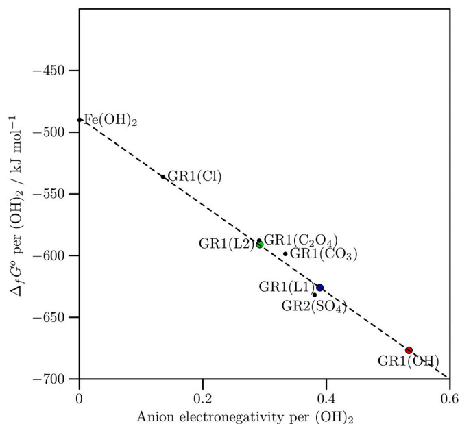
Fig. 6. Relationship between Gibbs free energies of formation of green rusts and fougèrite as a function of electronegativity of the interlayer anion. Filled black circles: measured values used to compute the linear regression, from Ben Nacib et al. (2016); red filled circle: estimated value for GR1-OH; blue and green filled circles: estimated values for GR1-lactate for the two structural formulas GR1-L1 and GR1-L2, from Sabot et al. (2007). (For interpretation of the references to colour in this figure legend, the reader is referred to the web version of this article.)
