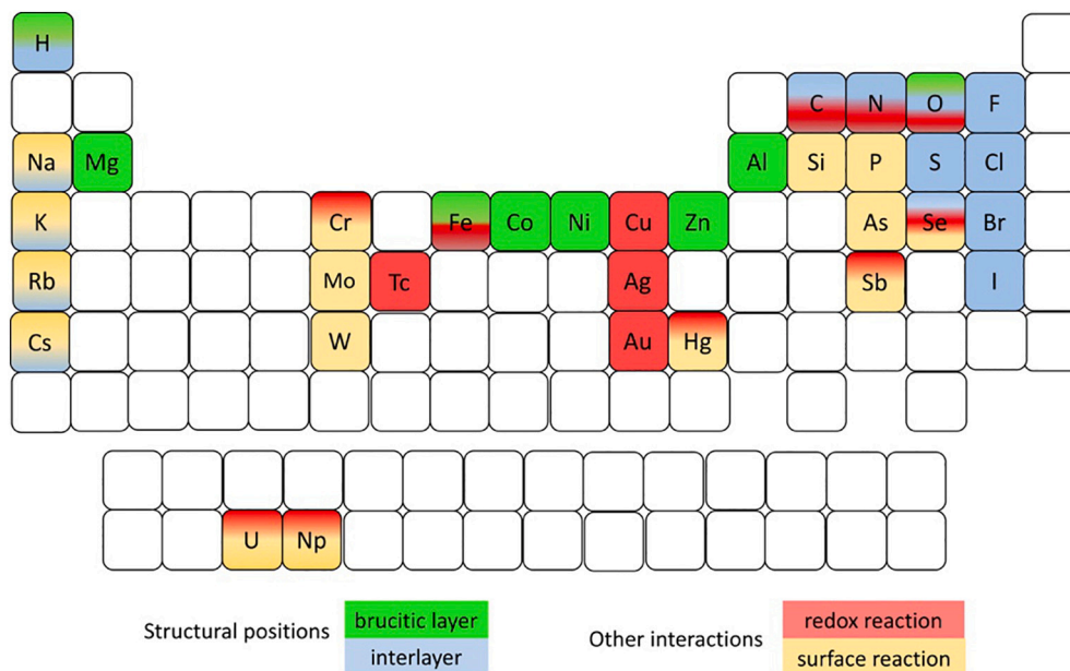
Fig. 8. Periodic table illustrating the possible interactions between green rusts and 34 elements through redox and surface reactions or surface exchange reactions, modified from Latta et al. (2015). (For interpretation of the references to colour in this figure legend, the reader is referred to the web version of this article.)
